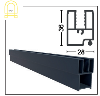
GYTN-1725 Dikey Baza 8 mm Vertical Base
