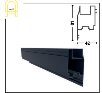
GYTN-1722 Açılır Kanat Isıcamlı Profile Of Insulated Opens
