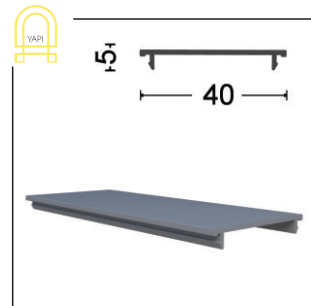
GYTN-1711 Yan Dikme Kapağı Side Cover Profile
