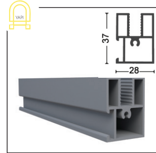
GYTN-1708 Baza 8 mm Profili Aluminum Glass Profile
