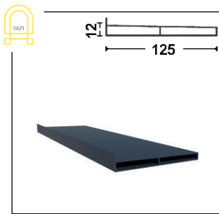
GYTN-1718 Alt Kasa Bottom Frame
