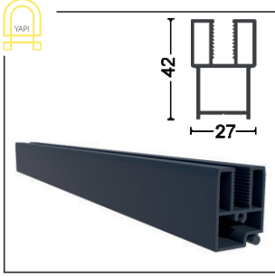
GYTN-1723 Alı-Üst Baza 8 mm Lower-Upper Base 8 mm
