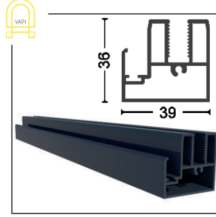
GYTN-1724 Çekme Baza 8 mm Pull Base 8 mm
