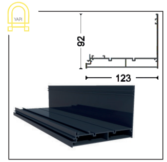
GYTN-1713 Yan Dikme Side Profile
