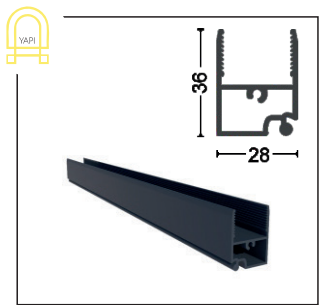
GYTN-1719 Alt-Üst Isıcamlı Baza Bottom-Top Insulating Glass Base
