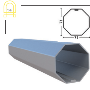
GYTN-2000 70'lik Sekizgen Sac Boru Octagonal Aluminum Tubing
