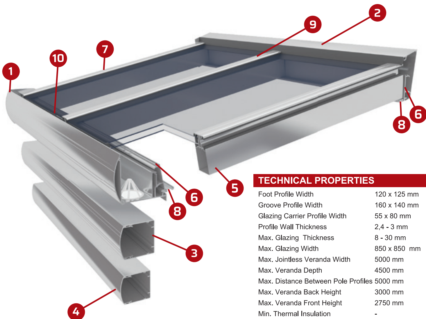
05 - Carrier Profile
